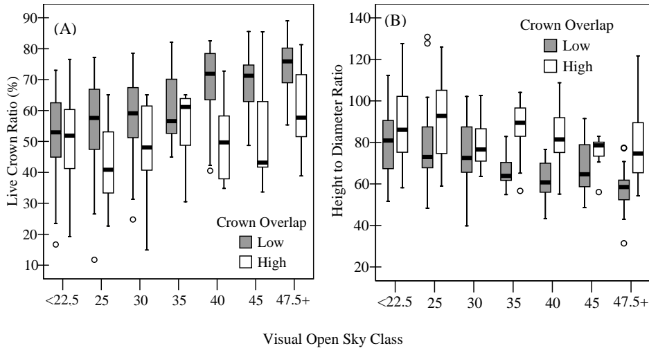
Figure 9: Boxplots of live crown ratio and height to diameter ratio for visual open sky classes for dominant and co-dominant trees in stand inventory (N=312). Classes are: <22.5, 22.6-27.5, 27.6-32.5, 32.6-37.5, 37.6-42.5, 42.5-47.5, 47.5+. Low crown overlap is <50% (2-dimensional), high crown overlap is 50%+ (2-dimensional).
