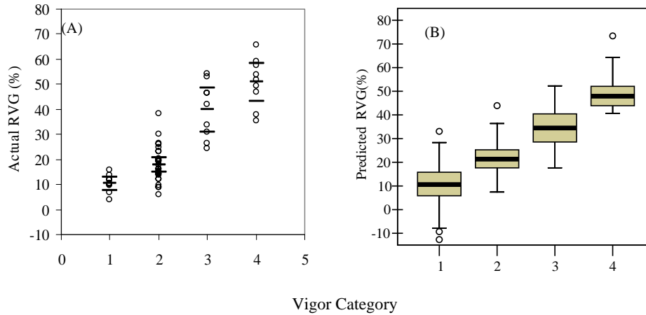
Figure 4: Vigor classes displayed against percent of maximum volume growth. Definitions of vigor classes are listed in table 2. (A) Scatterplot of 54 trees from phase 2. Means and 95% confidence intervals are displayed by hash marks. Means for all classes are significantly different from one another, Scheffe's post hoc test, ( p < .05 ). (B) Boxplot of 637 trees from phase 1. Means for all classes are significantly different from one other ( p < .0001 ).
