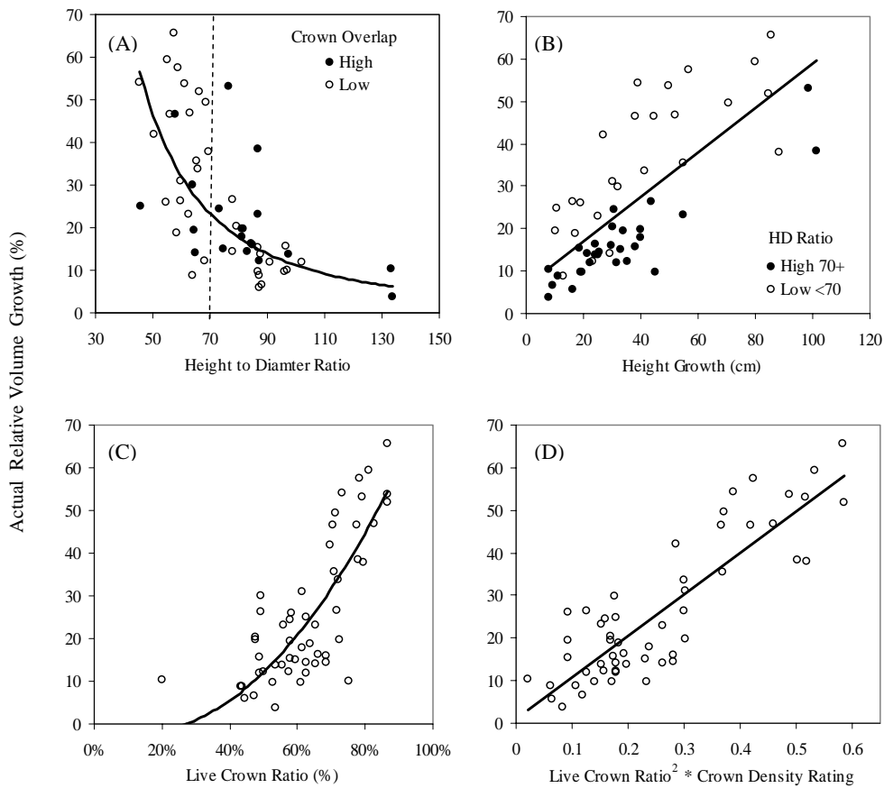
Figure 3: Scatterplots and fitted regression models of average of past 5yr relative volume growth. (A) Height to diameter ratio: the threshold of 70 is included for reference ( y=1481.950x - 2.016 , R^2=0.50 , SEE=0.476 , p<.0001 ). (B) Height growth annual increment, past 5yr average ( y=0.005x + 0.066 , R^2=0.55 , SEE=0.110 , p<.0001 ). (C) Live crown ratio ( y=1.054x^2 - 0.284x , R^2=0.64 , SEE=0.100 , p<.0001 ). (D) LCR^2 * Visual Crown Density Rating ( y=0.145x + 0.068 , R^2=0.76 , SEE=0.084 , p<.0001 ). N = 54 for all models.
