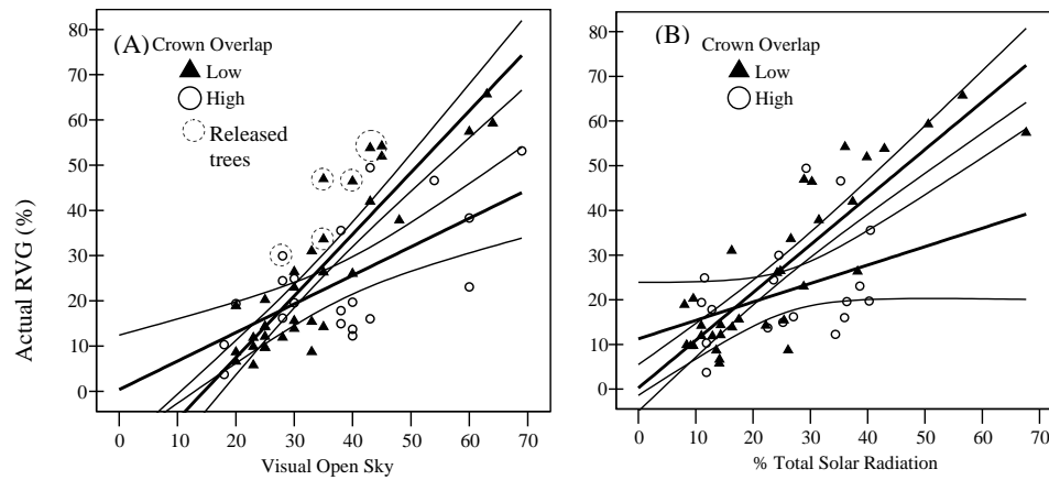
Figure 6: Fitted regression lines and 95% confidence intervals of actual RVG to measures of light for phase 2 trees. Three-dimensional crown overlap is included as a indicator ( d ) variable in regression models: low ( <30\%, 3d = 0 ), high ( 30\%+, 3d = 1 ). (A) Visual estimate of open sky ( N=54 , y=0.014x - 0.199 - 0.008dx + 0.207d , R^2 = 0.71 , SEE=0.092 , p<.0001 , all coefficients are significant p<.01 . R^2 = 0.79 for low crown overlap regression and R^2 = 0.43 for high crown overlap) (B) Percent of total solar radiation ( N=52 , y=0.011x + 0.003 - 0.007dx + 0.110d , R^2 = 0.65 , SEE=0.099 , p<.0001 , only slope coefficients are significant, p<.01 . R^2 = 0.75 for low crown overlap regression and R^2 = 0.18 for high crown overlap).
