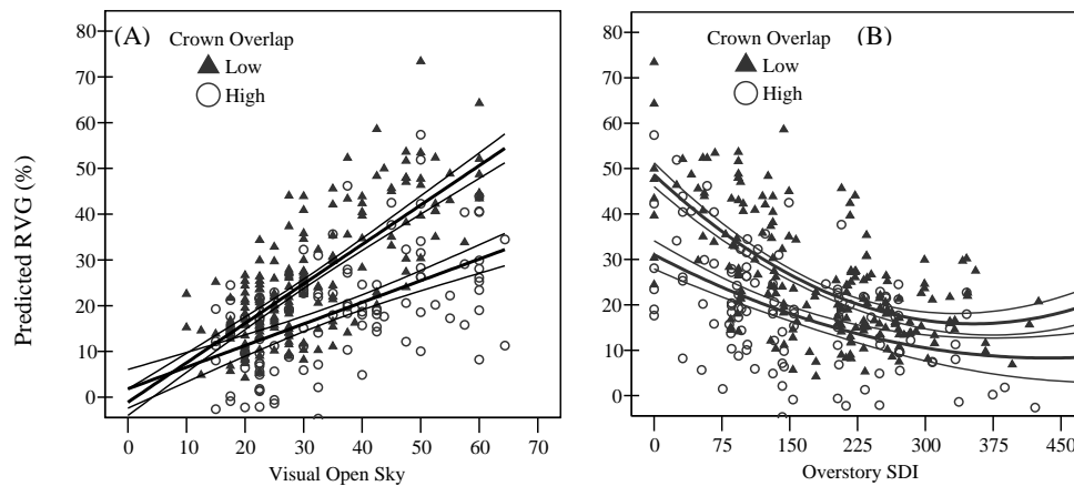
Figure 7: Fitted regression lines and 95% confidence intervals of predicted RVG to overstory measures for phase 1 crop trees (N=312). Crown overlap is included as an indicator ( d ) variable in regression models: low ( <50\%, 2d = 0 ), high ( 50\%+, 2d = 1 ). (A) Visual open sky ( y=.009x - 0.011 - 0.004dx + 0.027d , R^2 = 0.53 , SEE=0.090 , p<.0001 , only slope coefficients are significant p<.0001 . R^2 = 0.57 for low crown overlap regression and R^2 = 0.32 for high crown overlap) (B) Stand density index ( y = 0.0000027x^2 - 0.0000015dx^2 - 0.0019x + 0.000842dx + 0.487 - 0.179d , R^2 = 0.41 , SEE=0.103 , p<.0001 , all co-efficients are significant except for dx^2 , R^2 = 0.42 for low crown overlap regression and R^2 = 0.26 for high crown overlap)
