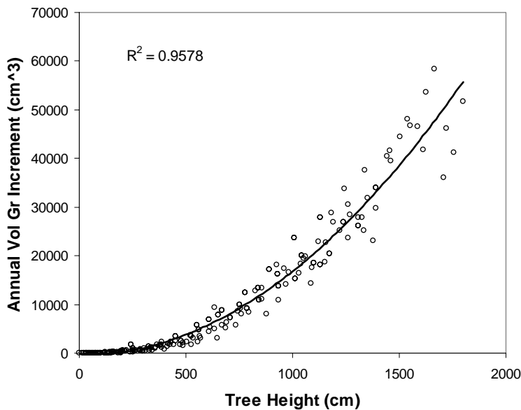
Figure 2: Scatterplot and fitted regression line for maximum site potential height (Ht) to volume growth curve. Each data point represents the annual volume growth increment for a single height of a tree. Multiple data points for each of the 19 trees are included y = 0.018x^2 - 0.27x - 466.74 ( R^2 = 0.96 , p < 0.0001 )
