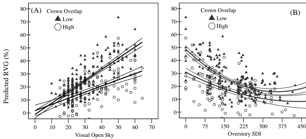
Figure S1: Fitted regression lines and 95% confidence intervals of predicted RVG to overstory measures for phase 1 crop trees (N=312). Crown overlap is included as an indicator ( d ) variable in regression models: low ( <50\%, 2d = 0 , high ( 50\%+, 2d = 1 ). (A) Visual open sky ( y = .009x - 0.011 - 0.004dx + 0.027d , R^2 = 0.53 , SEE = 0.090 , p < .0001 , only slope coefficients are significant p < .0001 . R^2 = 0.57 for low crown overlap regression and R^2 = 0.32 for high crown overlap.) (B) Stand density index ( y = 0.0000027x^2 - 0.0000015dx^2 - 0.0019x + 0.000842dx + 0.487 - 0.179d , R^2 = 0.41 , SEE = 0.103 , p < .0001 , all co-efficients are significant except for dx^2 , R^2 = 0.42 for low crown overlap regression and R^2 = 0.26 for high crown overlap).
